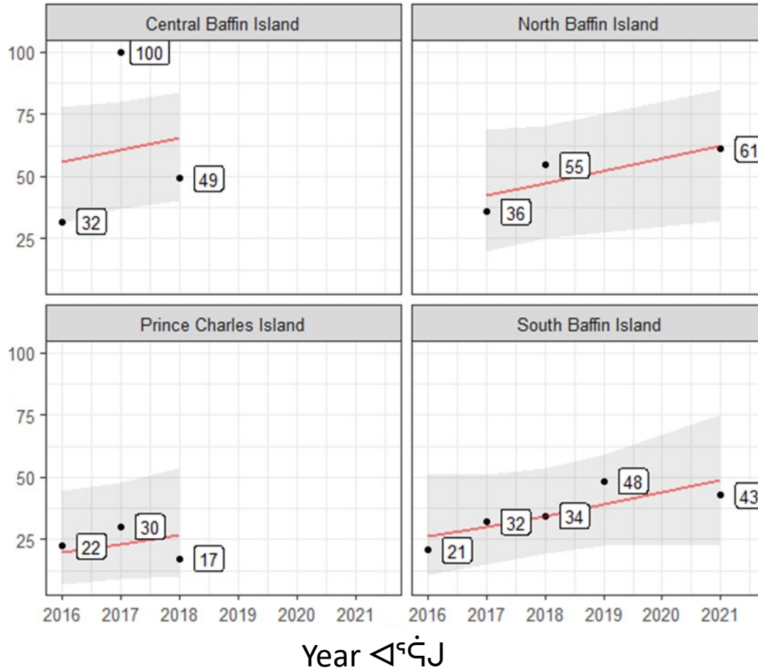
Spring calf-cow ratio \Delta \wedge \text{ᐅᐅᐅᐅᐅᐅ} \text{ᐅᐅᐅᐅᐅᐅᐅᐅᐅᐅᐅᐅᐅᐅ}
